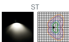
Street Optic
